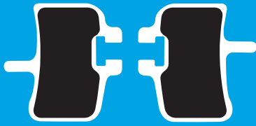
Org Sin 6850 6850 S COMPATIBLE WITH HAYES HFX-MAG SERIES / HFX 9 SERIES / MX1 AND PROMAX HYDR. LEFT / RIGHT PAD DIFFERENT SHAPE
